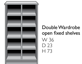
Double Wardrobe interior shelf with J-Bar W 36 D 23 H 73
