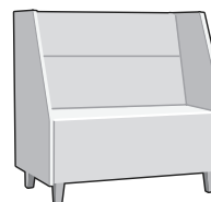
Curved outside 45° curve W 38.5 D 30 H 31.5 Seat H 18
